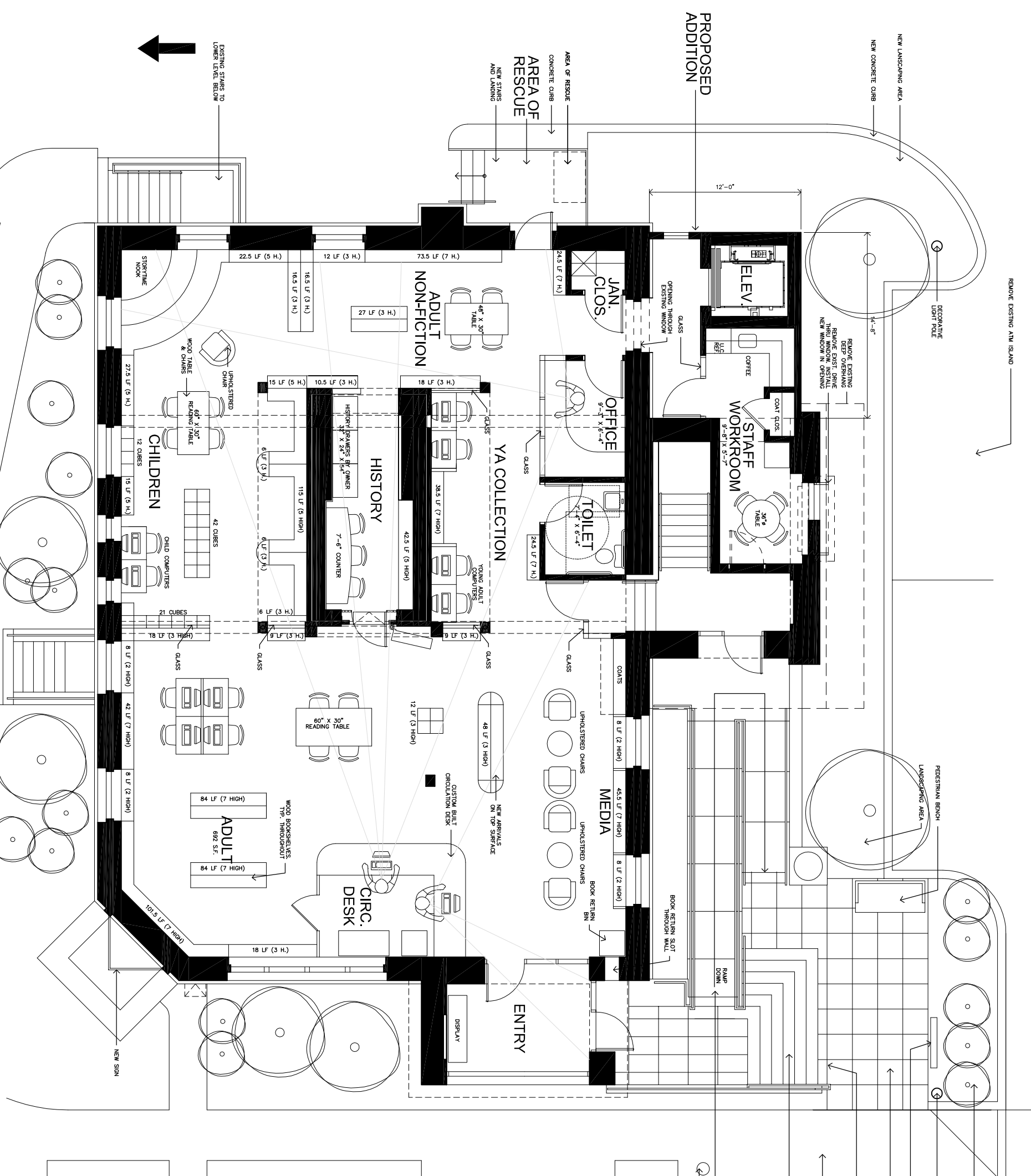
1 A.2 1/4" = 1'-0" MAIN LEVEL FLOOR PLAN PHASE 2
