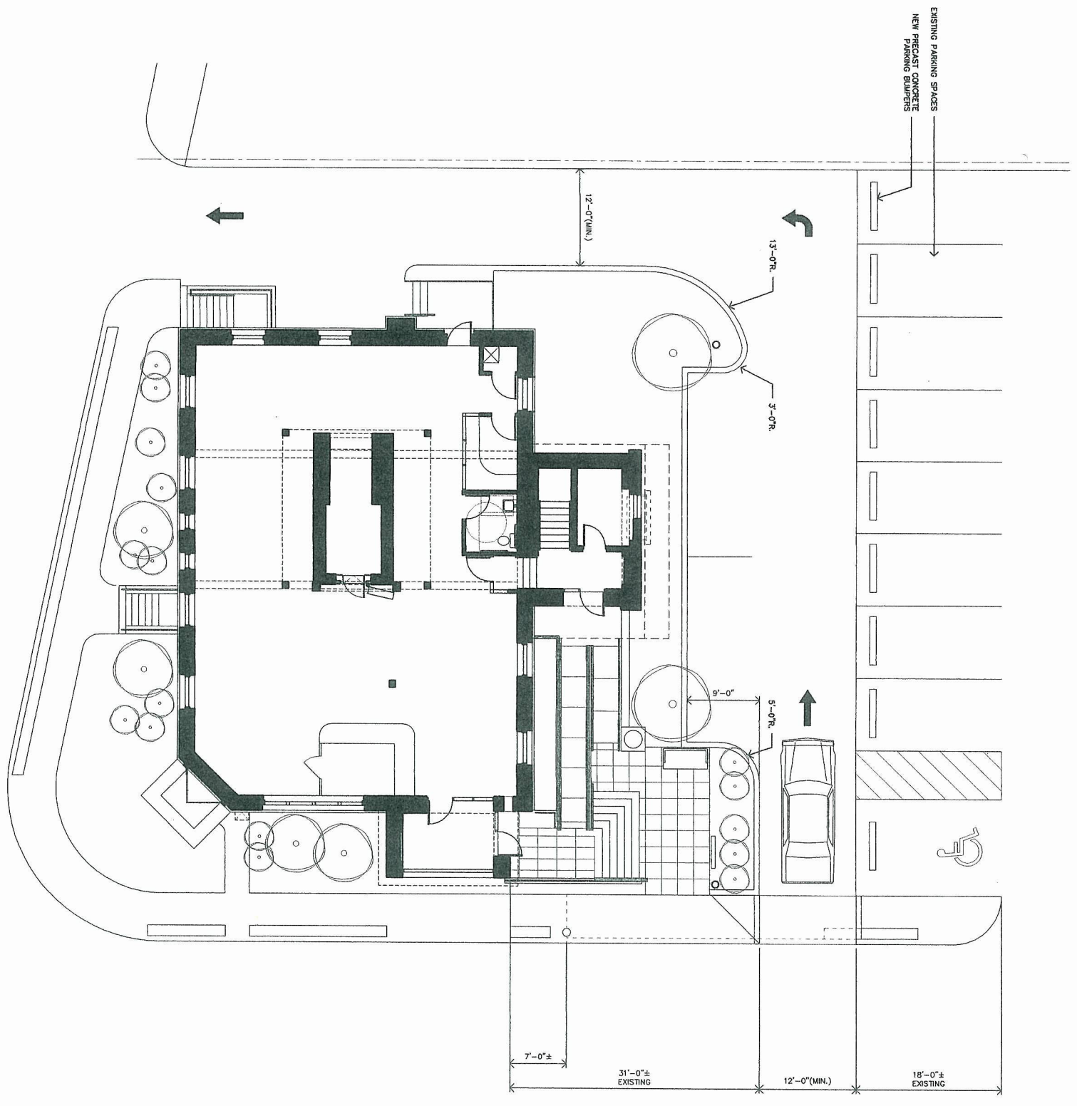
1 10ft 1/8" = 1'-0" SITE PLAN PHASE 1
